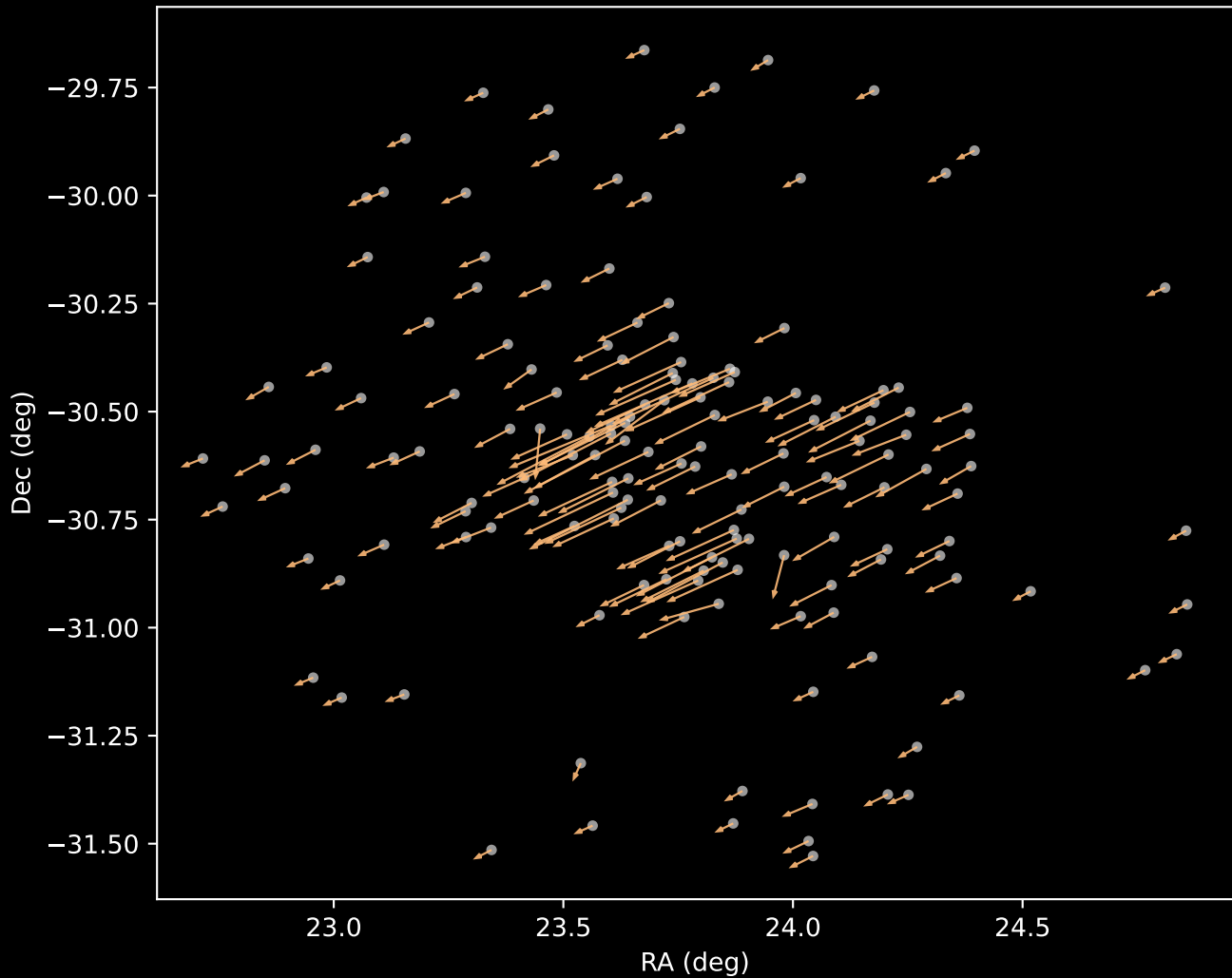
APOGEE DR17 Cluster 3 Proper Motion Vectors (n=160)
