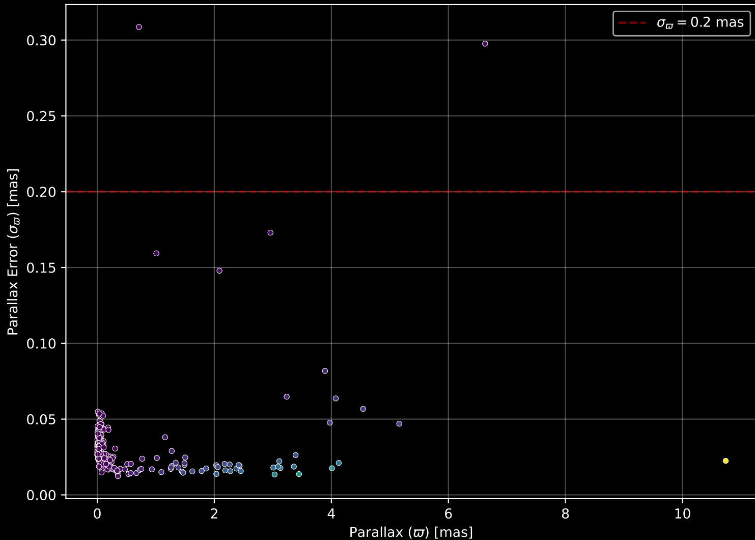
APOGEE DR17 Field: [M54SGRC1] Parallax Quality (n= 265)
