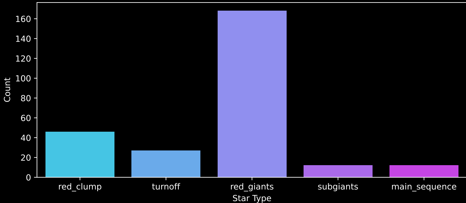
APOGEE DR17 Field: [M54SGRC1] Count plot of Star Type
