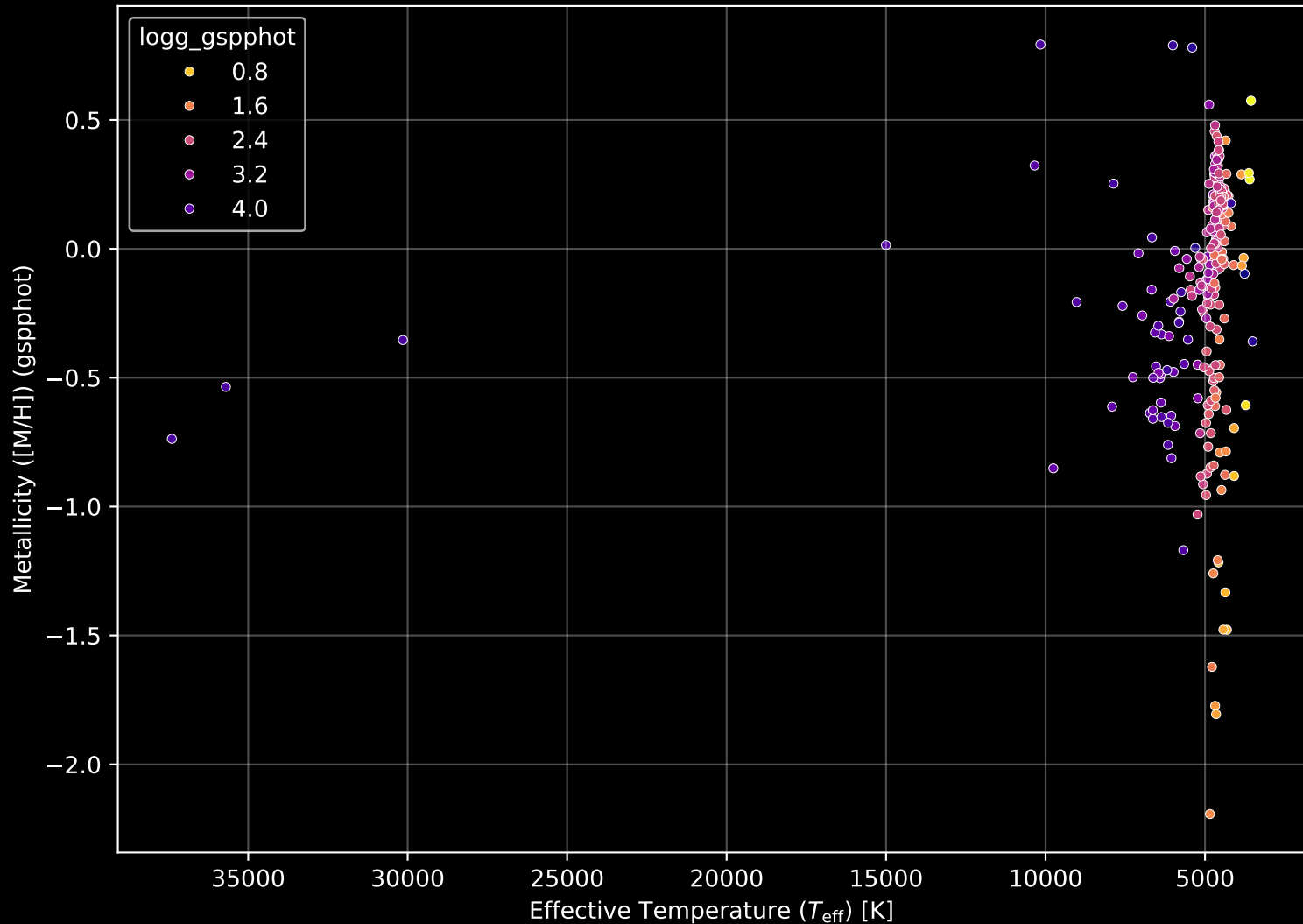
APOGEE DR17 Field: [M54SGRC1] Stellar Population Parameters (n= 265)
