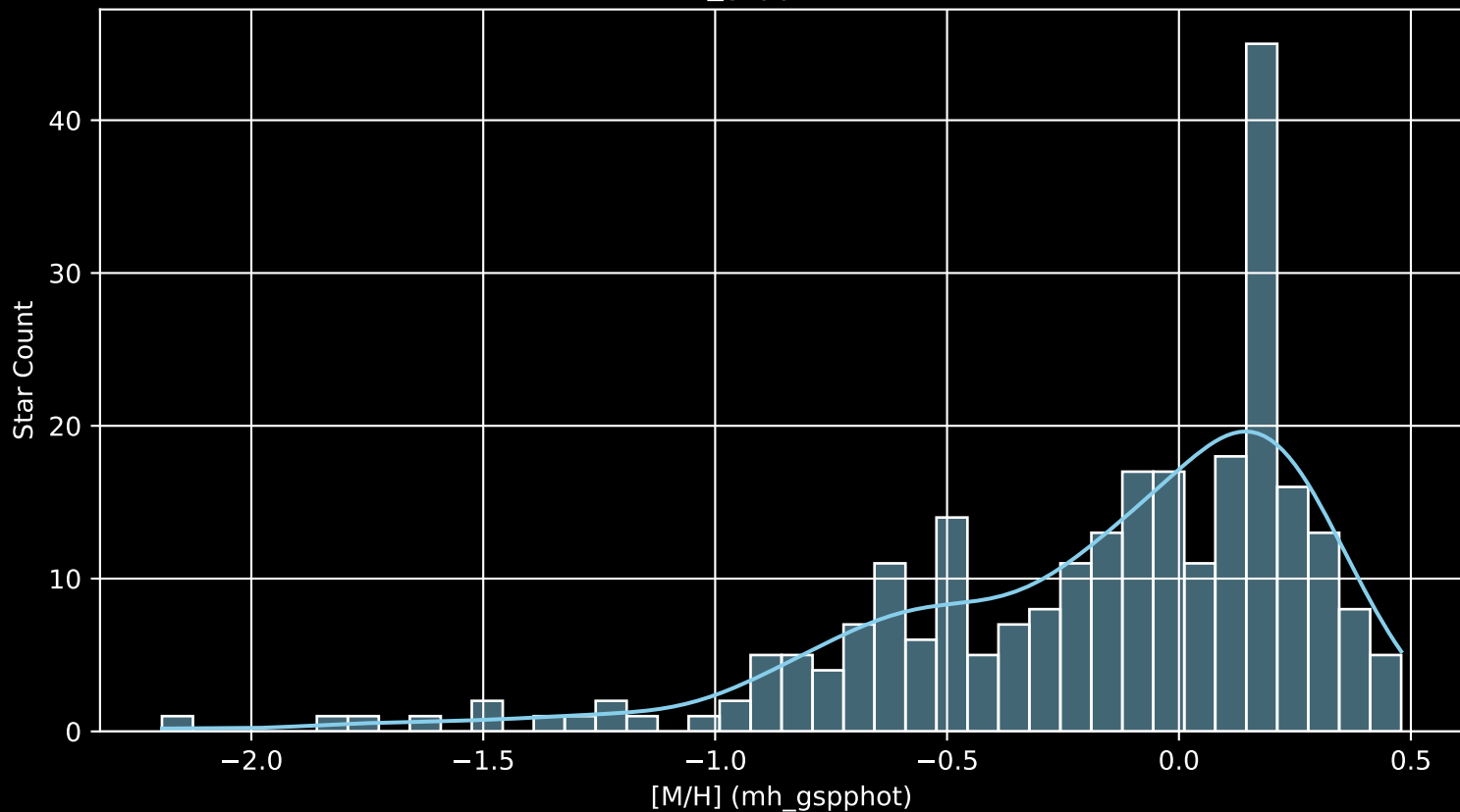
APOGEE DR17 Field: [M54SGRC1 [M/H] (mh_gspphot) (n= 260)
