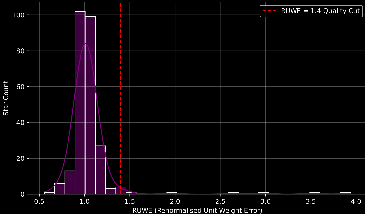
GAPOGEE DR17 Field [M54SGRC1] RUWE Distribution (n= 261)
