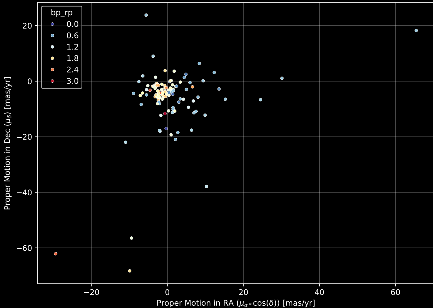
APOGEE DR17 Field: [M54SGRC1] Proper Motion Diagram (n= 265)
